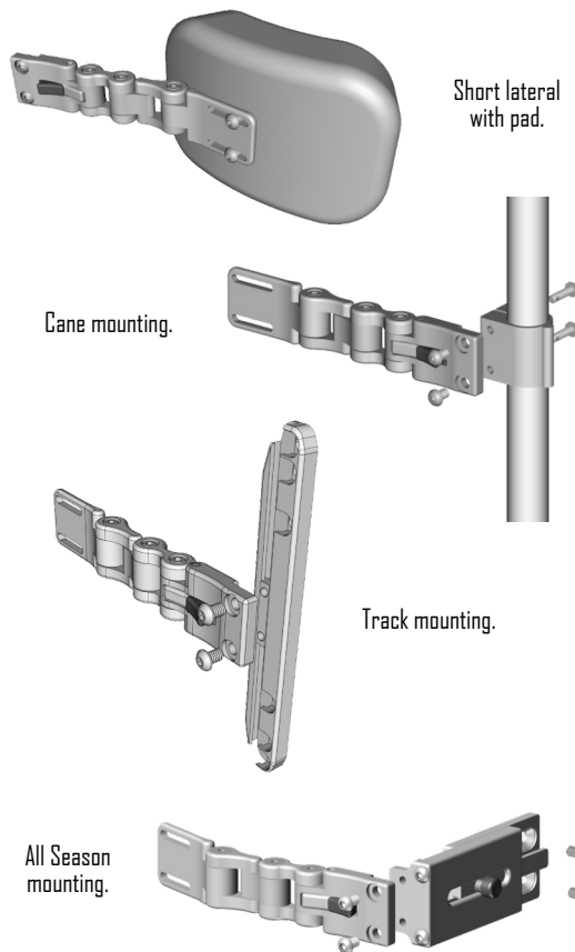
UIMBK1090 90° Bracket
